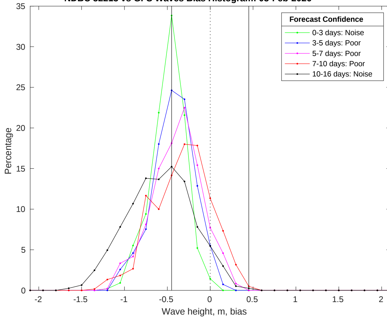
NDBC 52213 vs GFS Waves Bias Histogram: 03-Feb-2026
