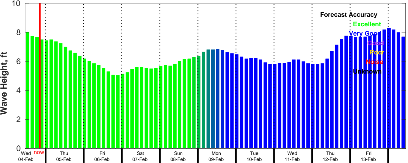
CMEMS Wave Forecast for NDBC 52213 from 03-Feb-2026 11:00:00 to 13-Feb-2026 11:00:00
