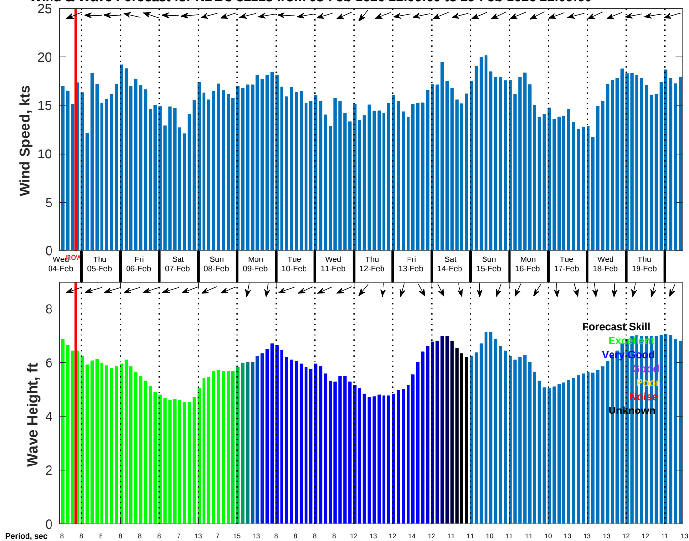
Wind & Wave Forecast for NDBC 52213 from 03-Feb-2026 11:00:00 to 19-Feb-2026 11:00:00
