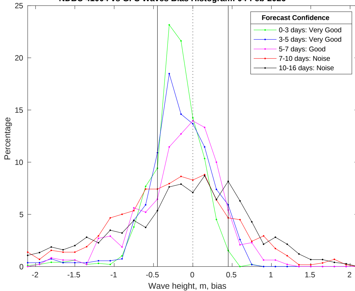
NDBC 41004 vs GFS Waves Bias Histogram: 04-Feb-2026
