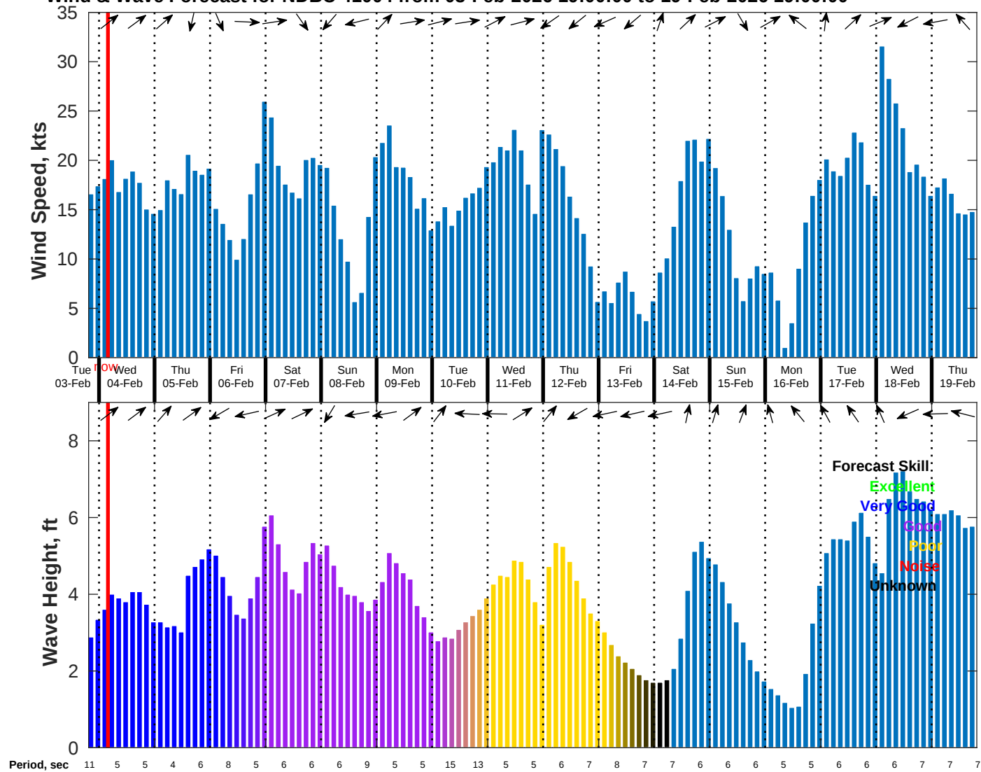
Wind & Wave Forecast for NDBC 41004 from 03-Feb-2026 19:00:00 to 19-Feb-2026 19:00:00
