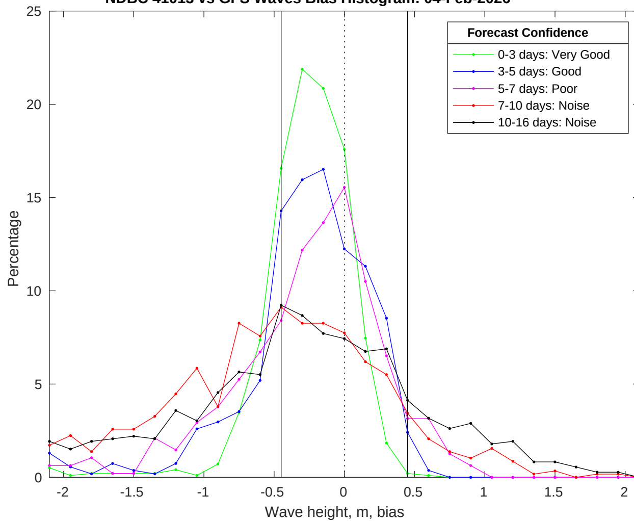
NDBC 41013 vs GFS Waves Bias Histogram: 04-Feb-2026
