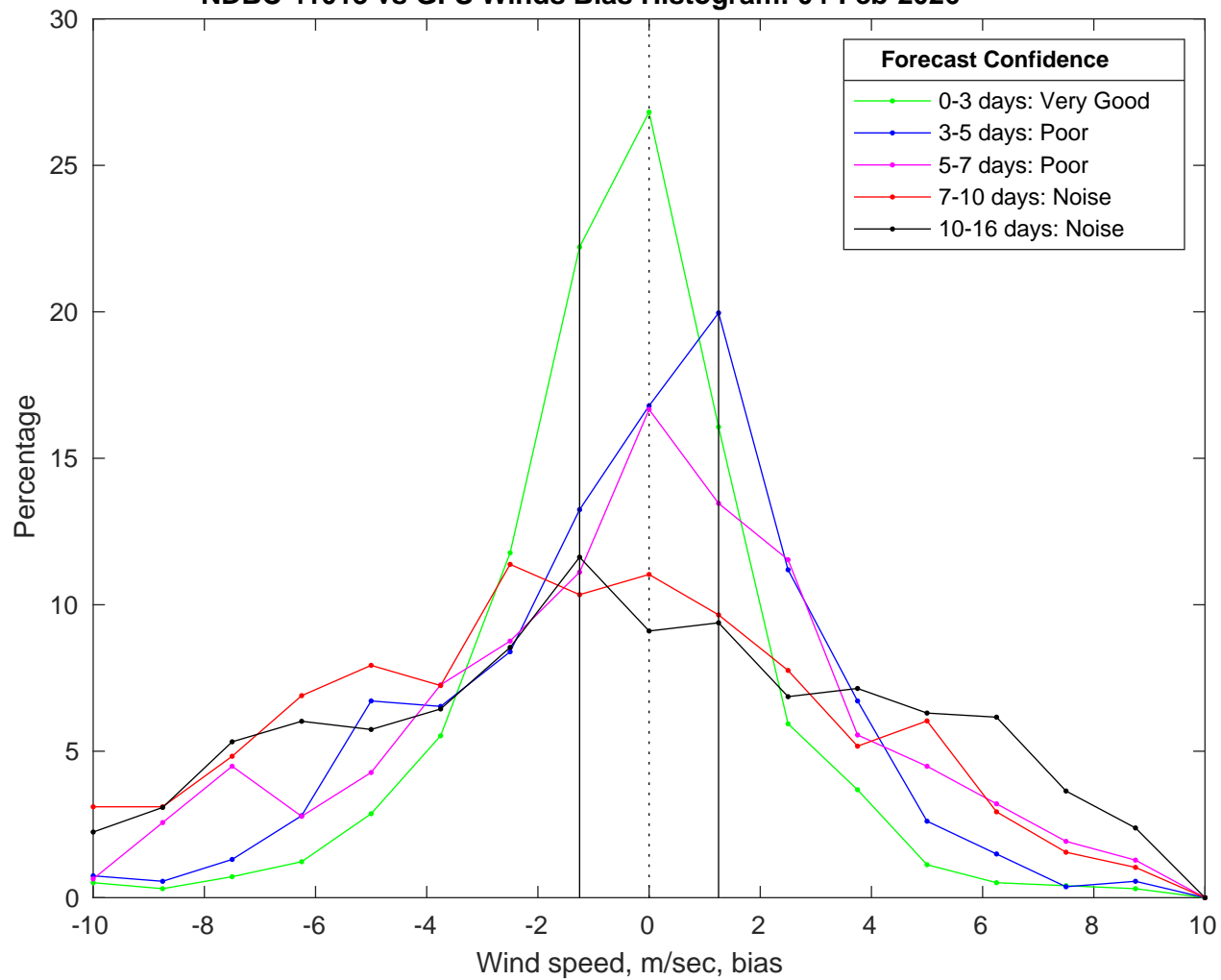
NDBC 41013 vs GFS Winds Bias Histogram: 04-Feb-2026
