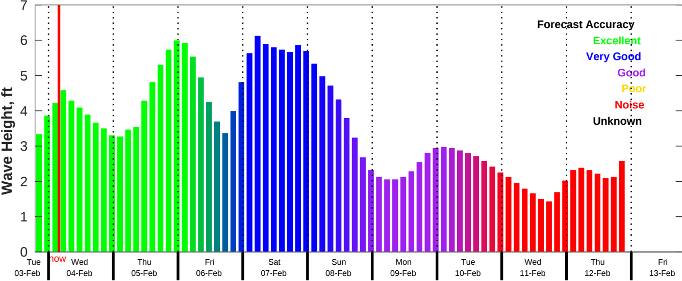
CMEMS Wave Forecast for NDBC 41013 from 03-Feb-2026 19:00:00 to 13-Feb-2026 19:00:00
