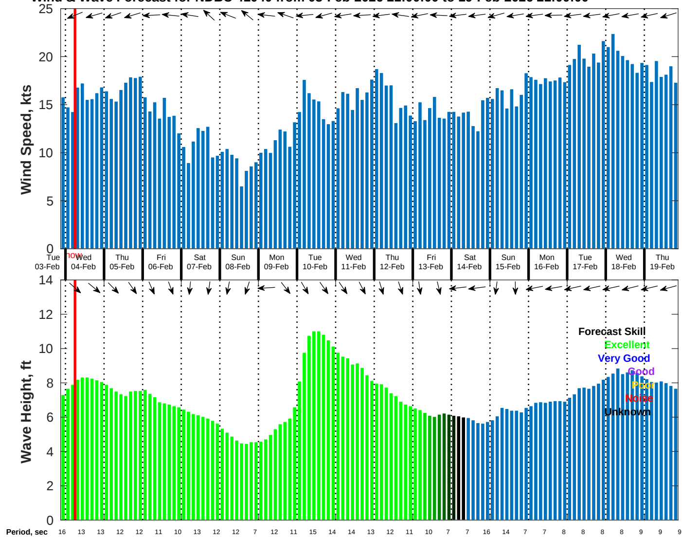
Wind & Wave Forecast for NDBC 41040 from 03-Feb-2026 21:00:00 to 19-Feb-2026 21:00:00
