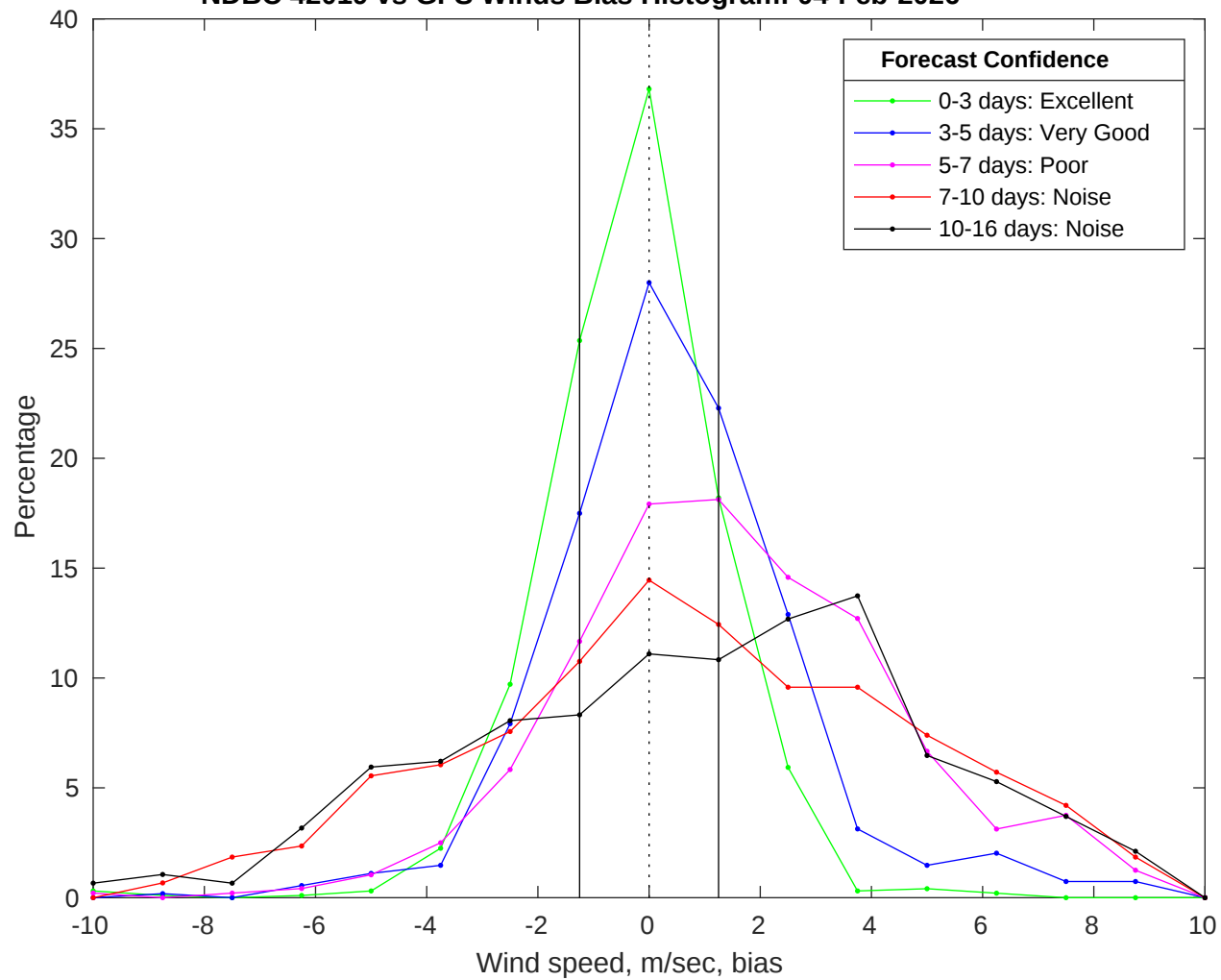
NDBC 42019 vs GFS Winds Bias Histogram: 04-Feb-2026
