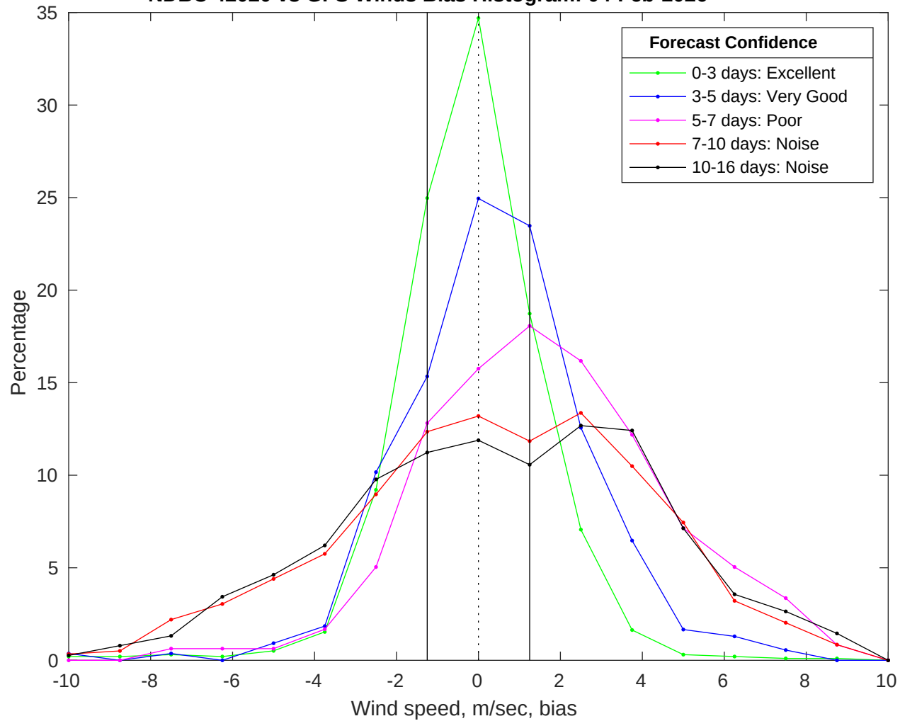
NDBC 42020 vs GFS Winds Bias Histogram: 04-Feb-2026
