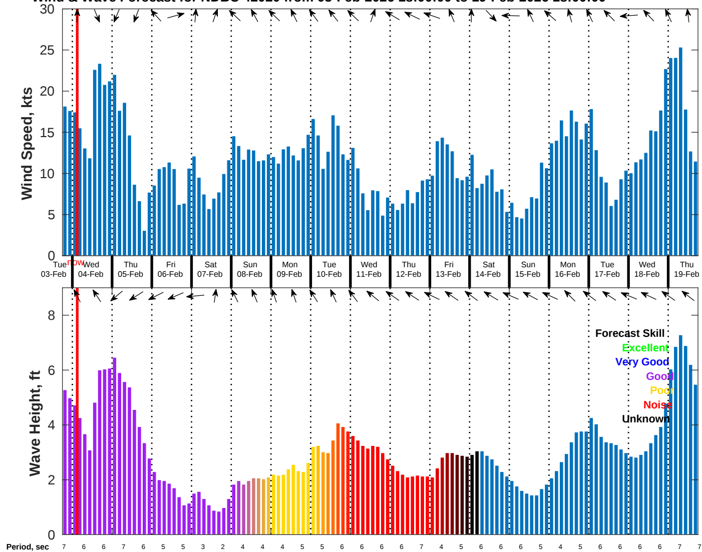
Wind & Wave Forecast for NDBC 42020 from 03-Feb-2026 18:00:00 to 19-Feb-2026 18:00:00
