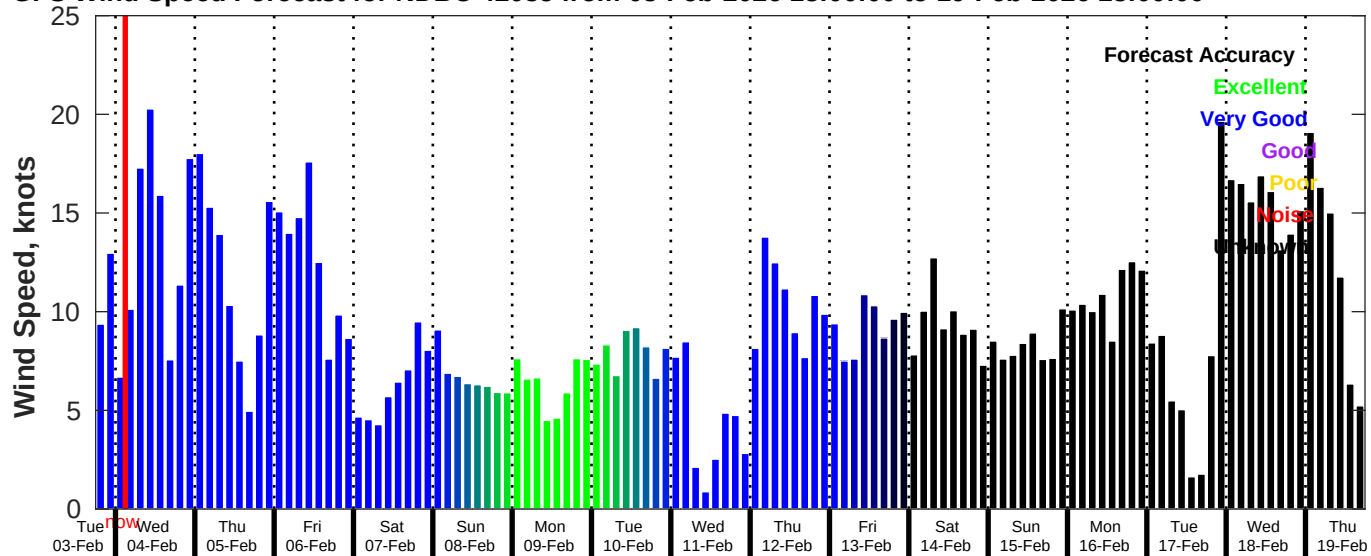
GFS Wind Speed Forecast for NDBC 42035 from 03-Feb-2026 18:00:00 to 19-Feb-2026 18:00:00
