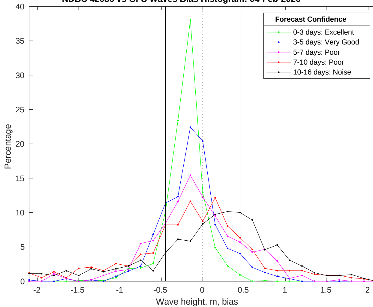
NDBC 42036 vs GFS Waves Bias Histogram: 04-Feb-2026
