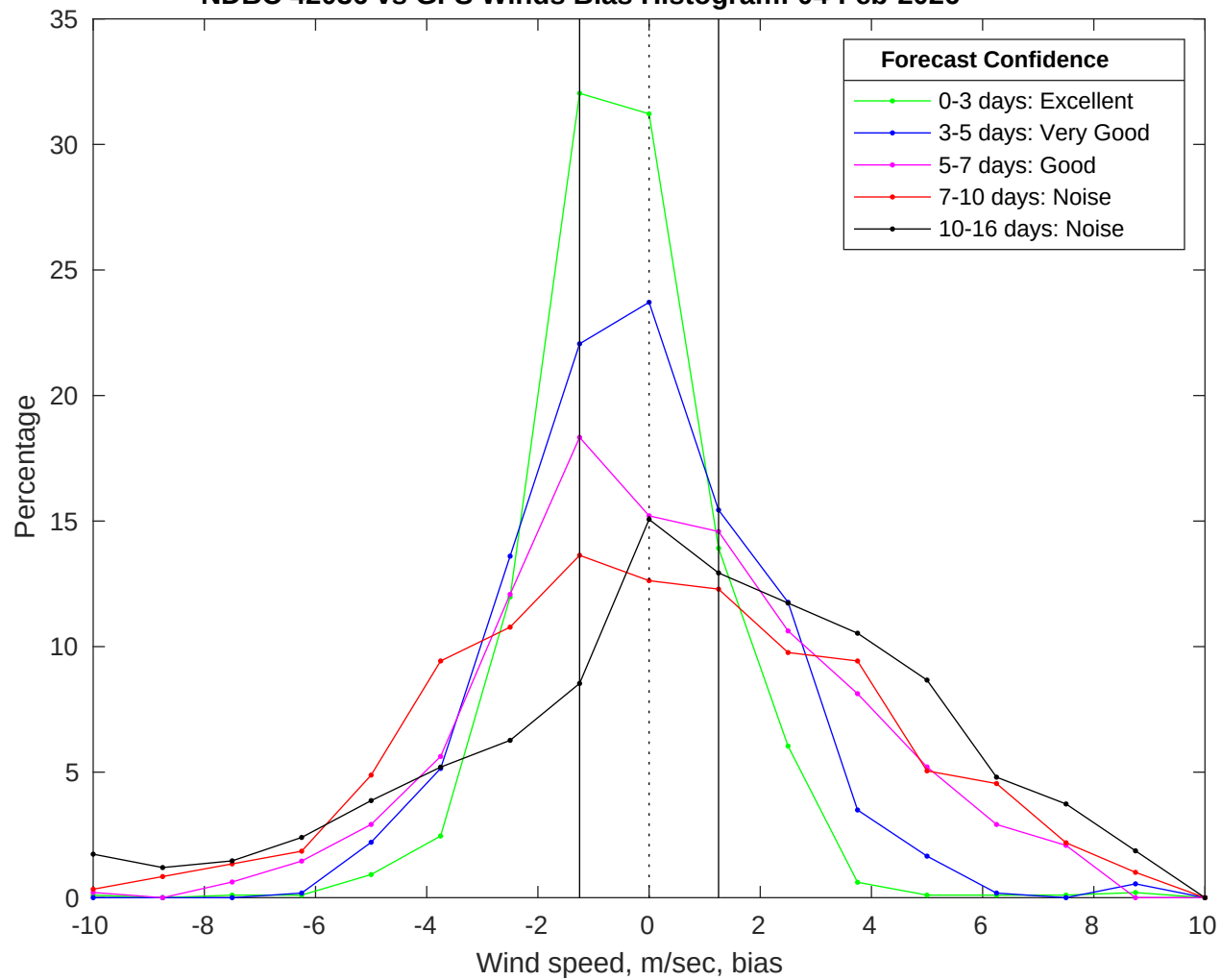
NDBC 42036 vs GFS Winds Bias Histogram: 04-Feb-2026
