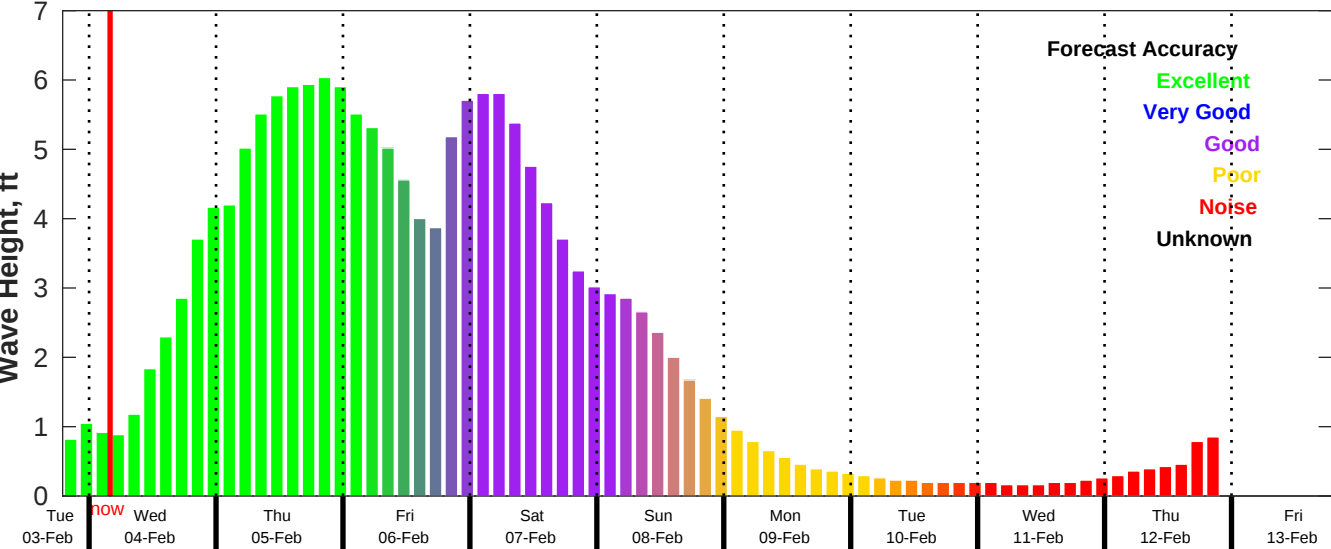
CMEMS Wave Forecast for NDBC 42036 from 03-Feb-2026 19:00:00 to 13-Feb-2026 19:00:00
