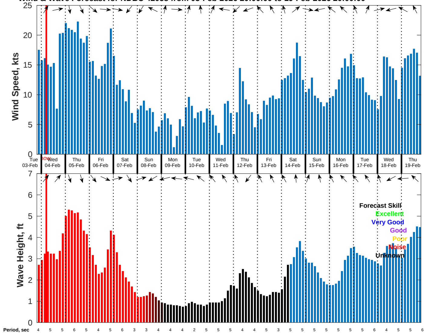
Wind & Wave Forecast for NDBC 42058 from 03-Feb-2026 20:00:00 to 19-Feb-2026 20:00:00
