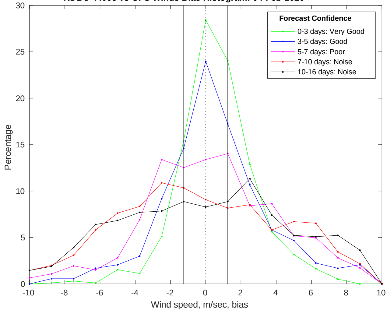
NDBC 44008 vs GFS Winds Bias Histogram: 04-Feb-2026
