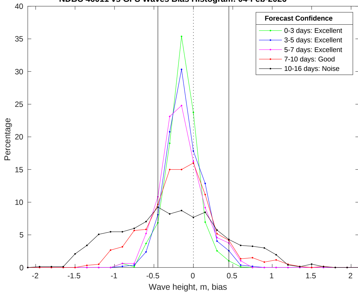
NDBC 46011 vs GFS Waves Bias Histogram: 04-Feb-2026
