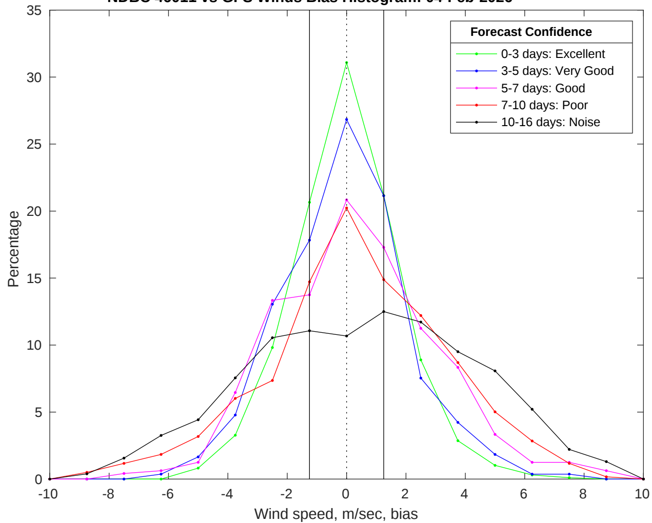
NDBC 46011 vs GFS Winds Bias Histogram: 04-Feb-2026
