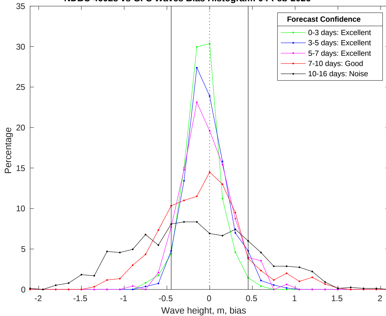
NDBC 46028 vs GFS Waves Bias Histogram: 04-Feb-2026
