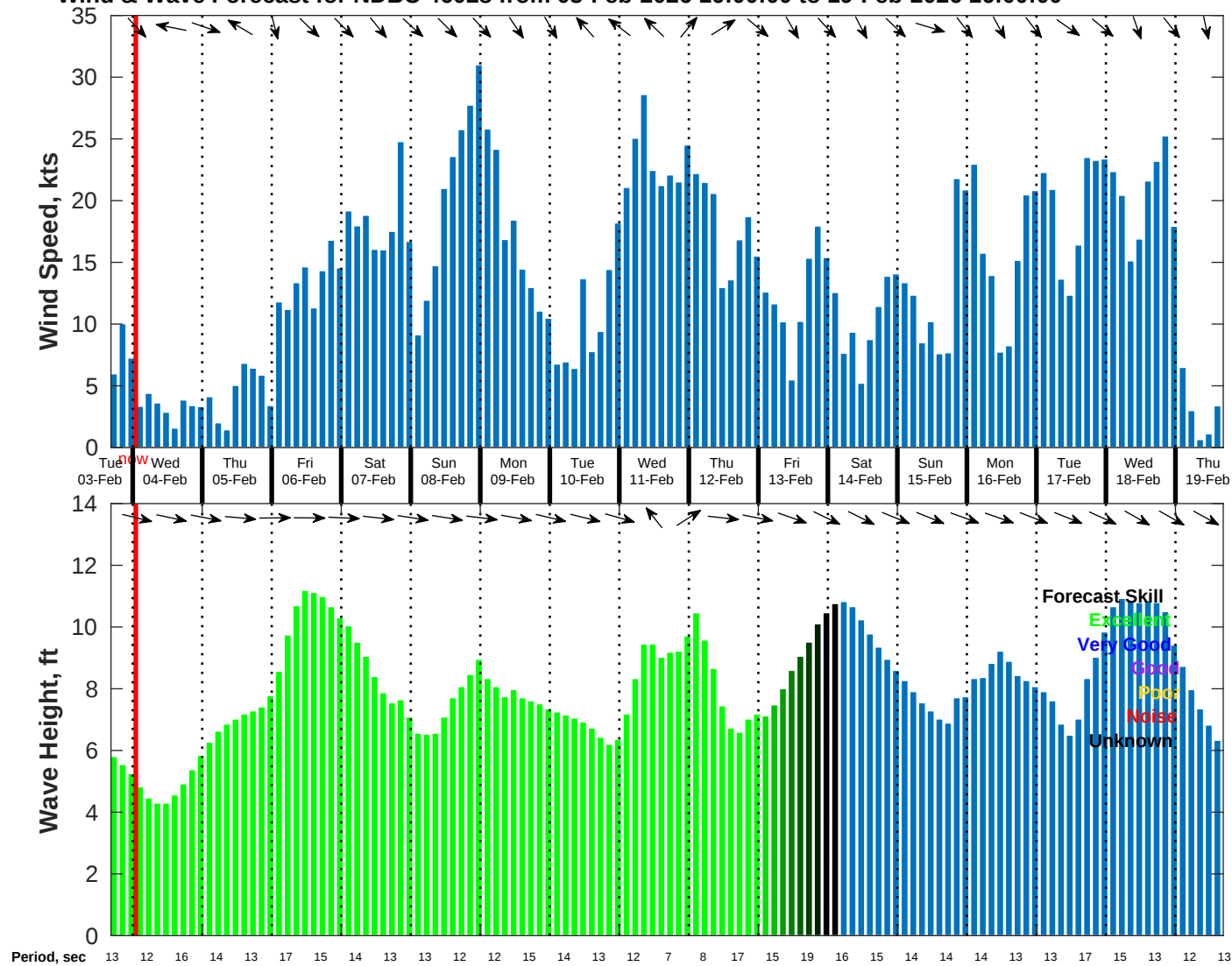
Wind & Wave Forecast for NDBC 46028 from 03-Feb-2026 16:00:00 to 19-Feb-2026 16:00:00
