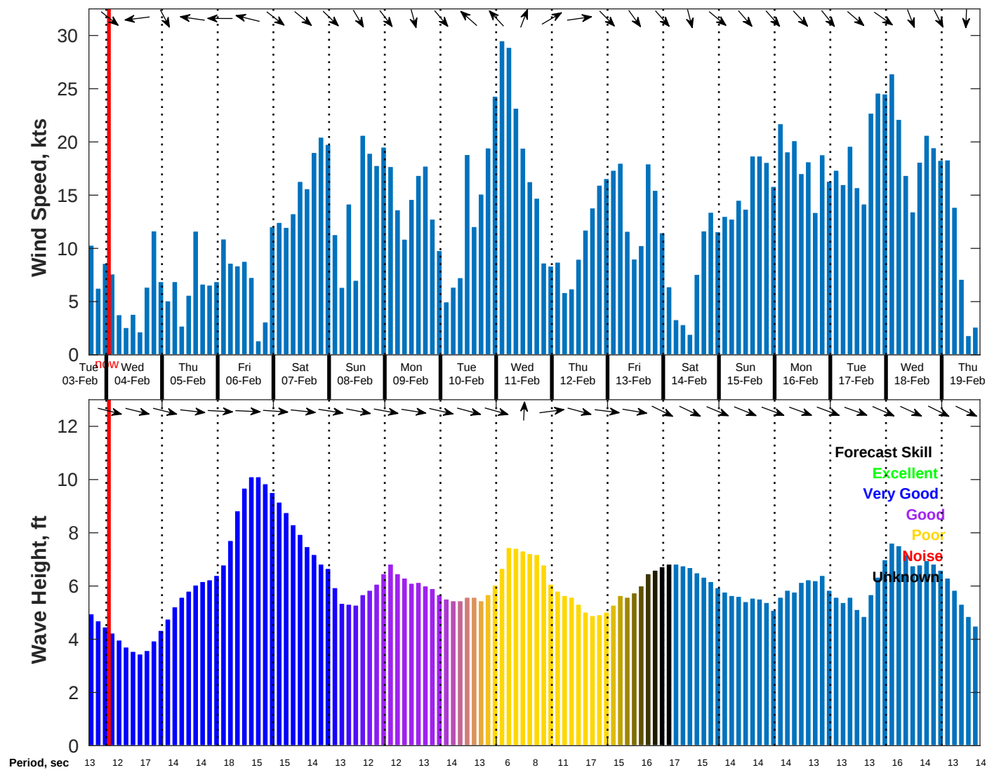
Wind & Wave Forecast for NDBC 46054 from 03-Feb-2026 16:00:00 to 19-Feb-2026 16:00:00
