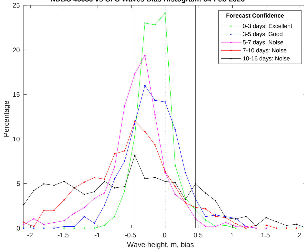
NDBC 46059 vs GFS Waves Bias Histogram: 04-Feb-2026
