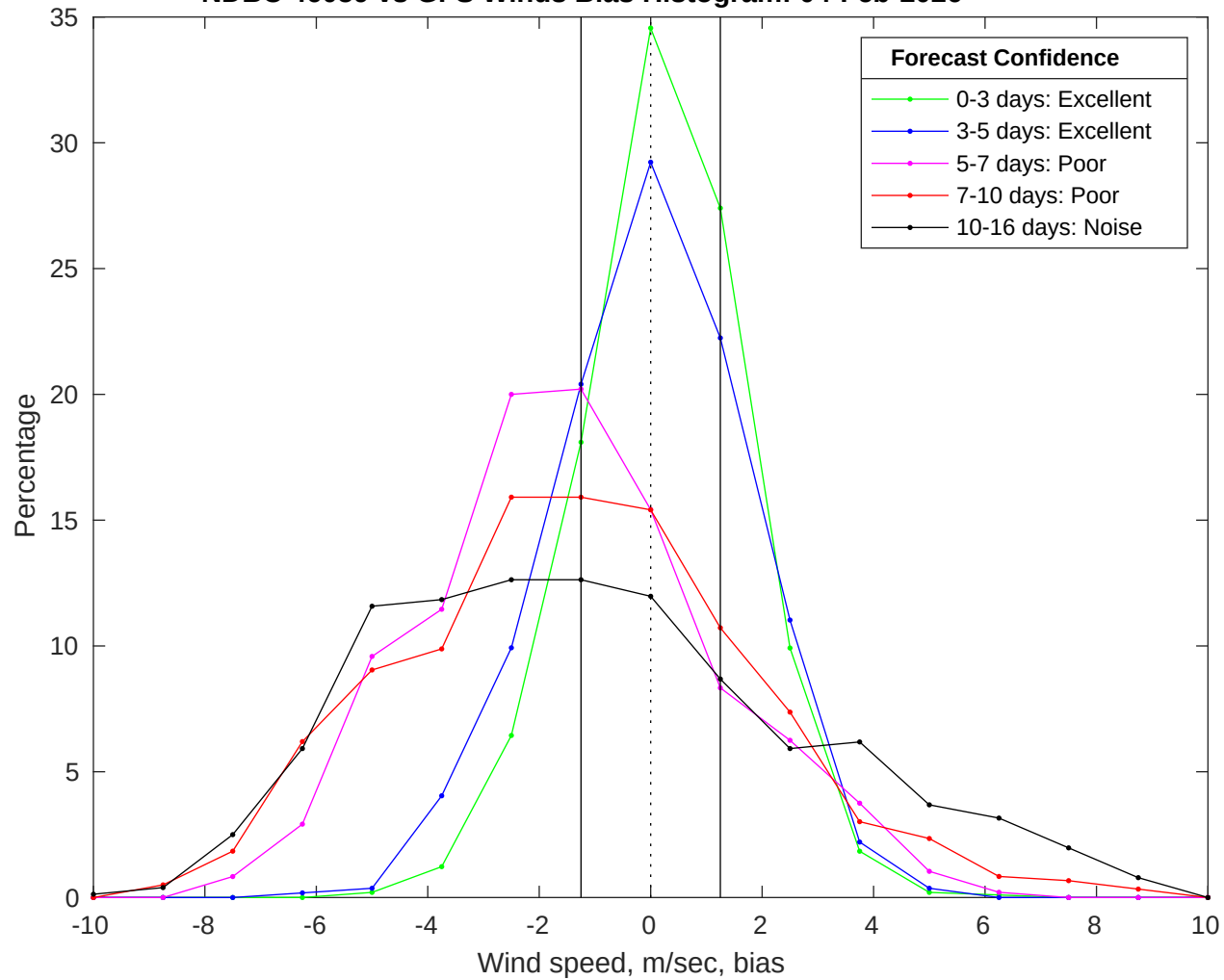
NDBC 46059 vs GFS Winds Bias Histogram: 04-Feb-2026
