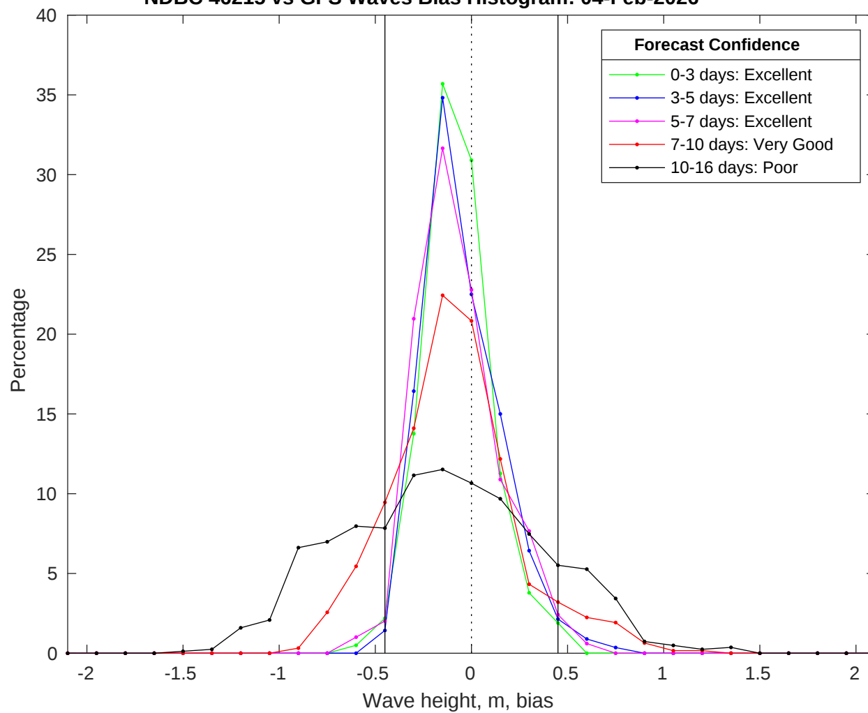
NDBC 46215 vs GFS Waves Bias Histogram: 04-Feb-2026
