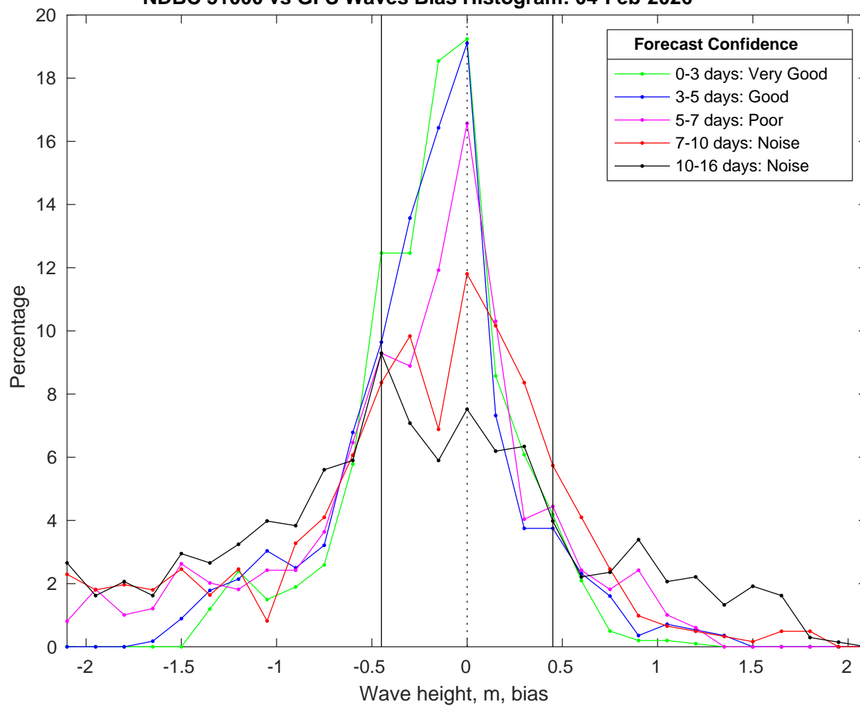
NDBC 51000 vs GFS Waves Bias Histogram: 04-Feb-2026
