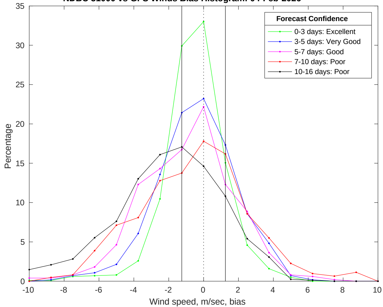
NDBC 51000 vs GFS Winds Bias Histogram: 04-Feb-2026
