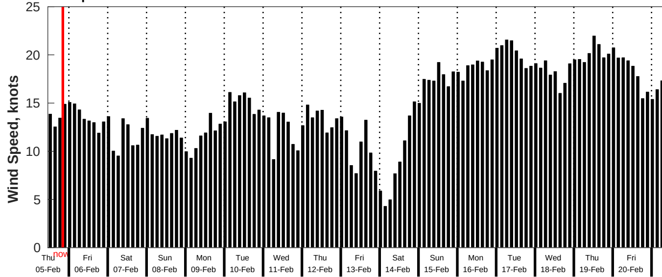
GFS Wind Speed Forecast for NDBC 52211 from 04-Feb-2026 11:00:00 to 20-Feb-2026 11:00:00
