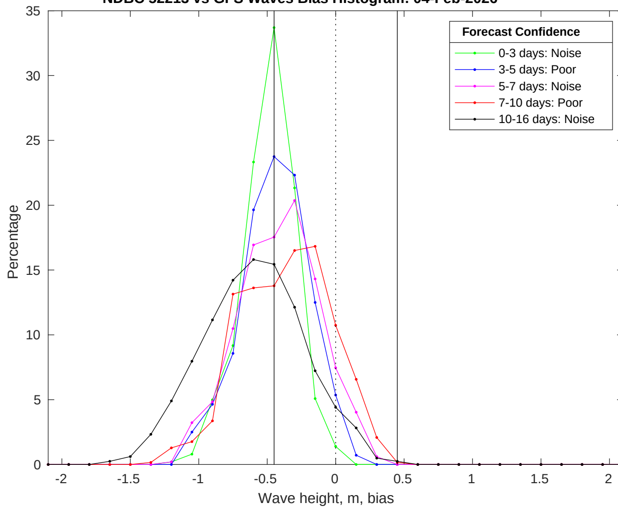
NDBC 52213 vs GFS Waves Bias Histogram: 04-Feb-2026
