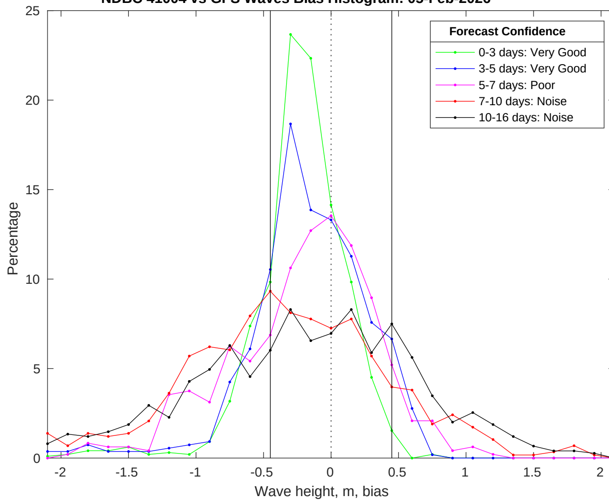
NDBC 41004 vs GFS Waves Bias Histogram: 05-Feb-2026
