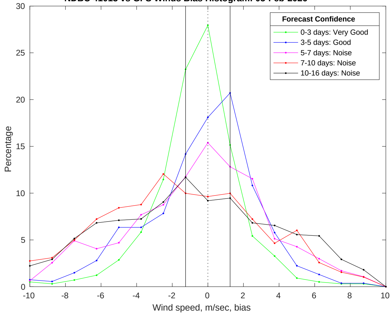
NDBC 41013 vs GFS Winds Bias Histogram: 05-Feb-2026
