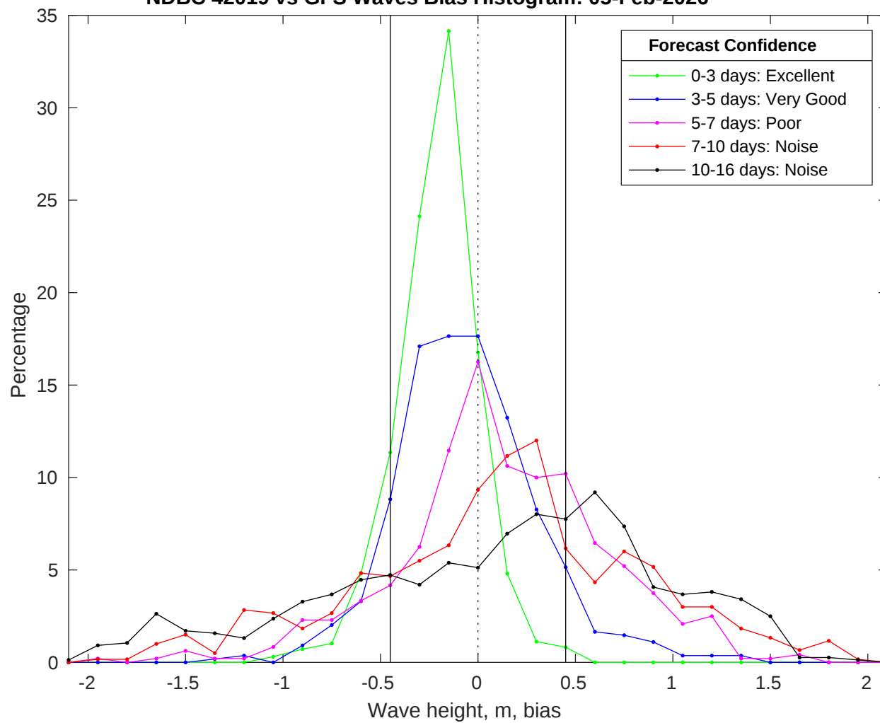
NDBC 42019 vs GFS Waves Bias Histogram: 05-Feb-2026
