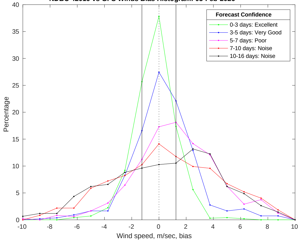
NDBC 42019 vs GFS Winds Bias Histogram: 05-Feb-2026
