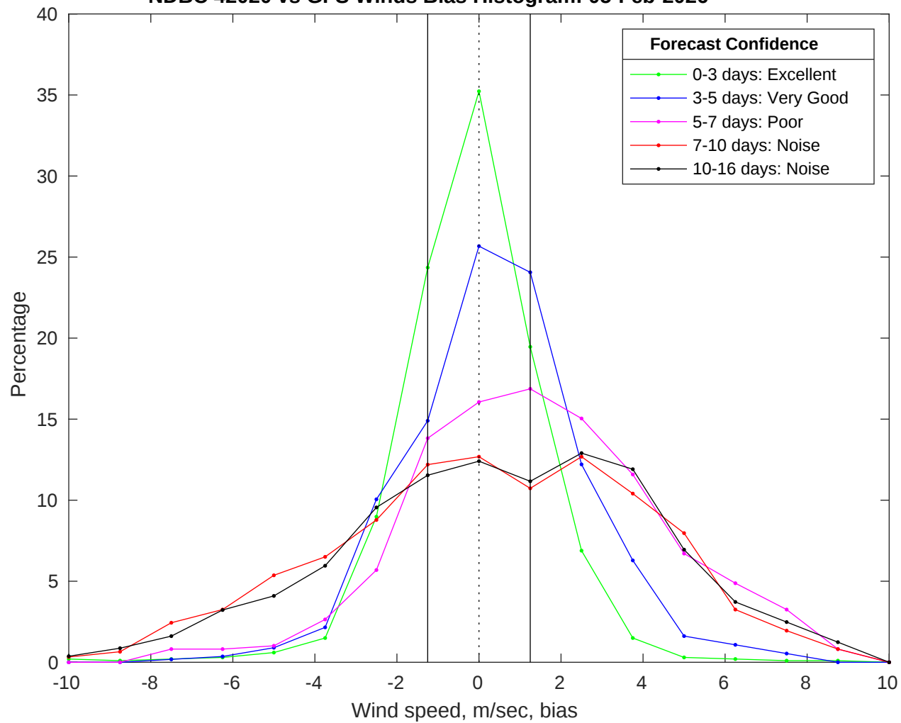
NDBC 42020 vs GFS Winds Bias Histogram: 05-Feb-2026
