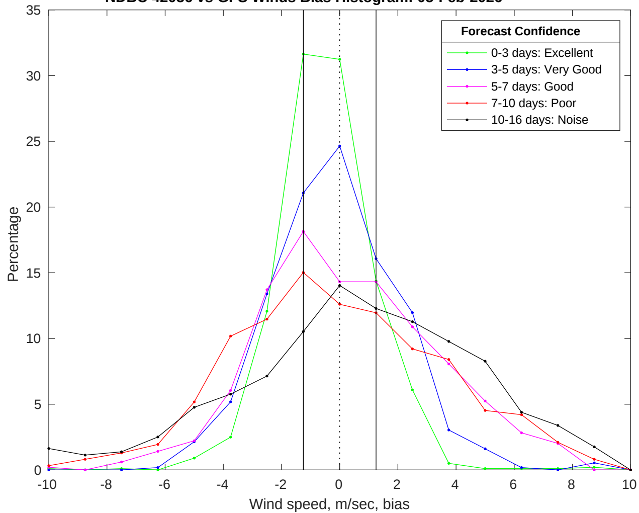
NDBC 42036 vs GFS Winds Bias Histogram: 05-Feb-2026
