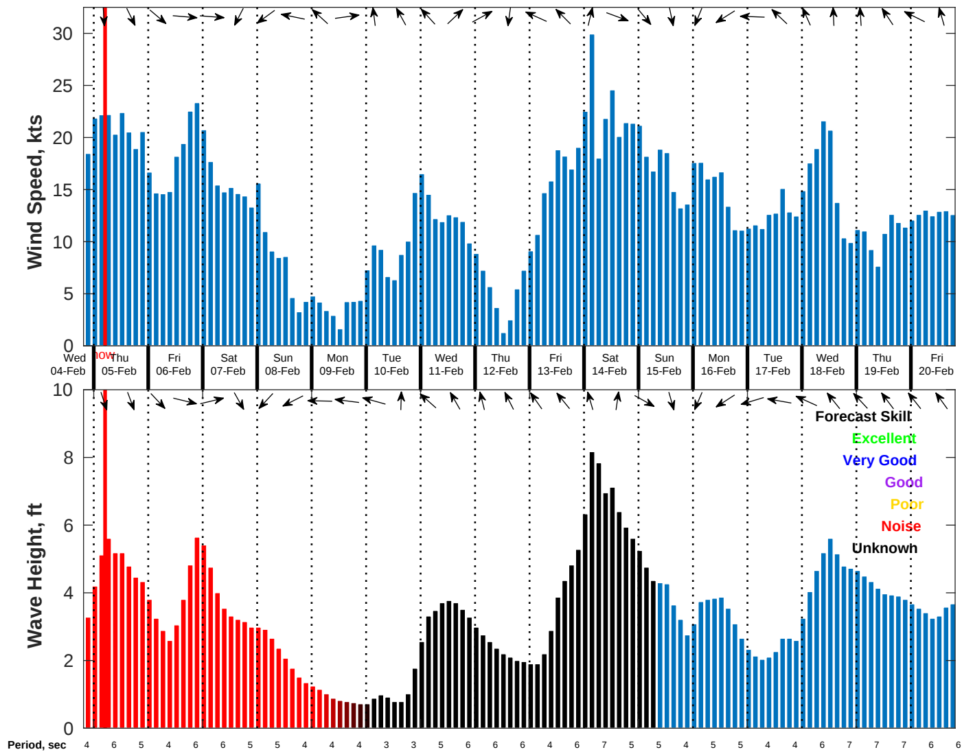
Wind & Wave Forecast for NDBC 42058 from 04-Feb-2026 20:00:00 to 20-Feb-2026 20:00:00
