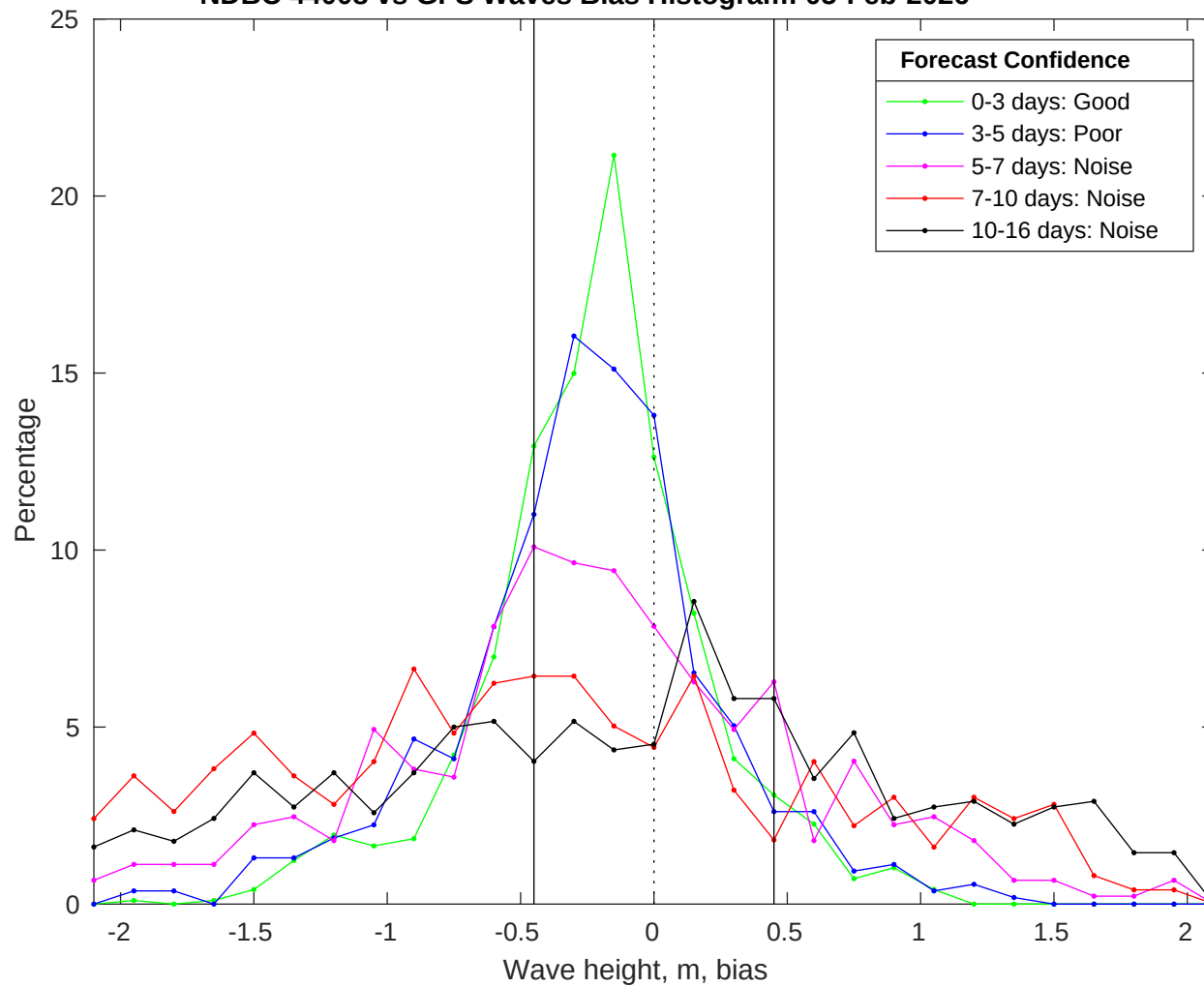
NDBC 44008 vs GFS Waves Bias Histogram: 05-Feb-2026
