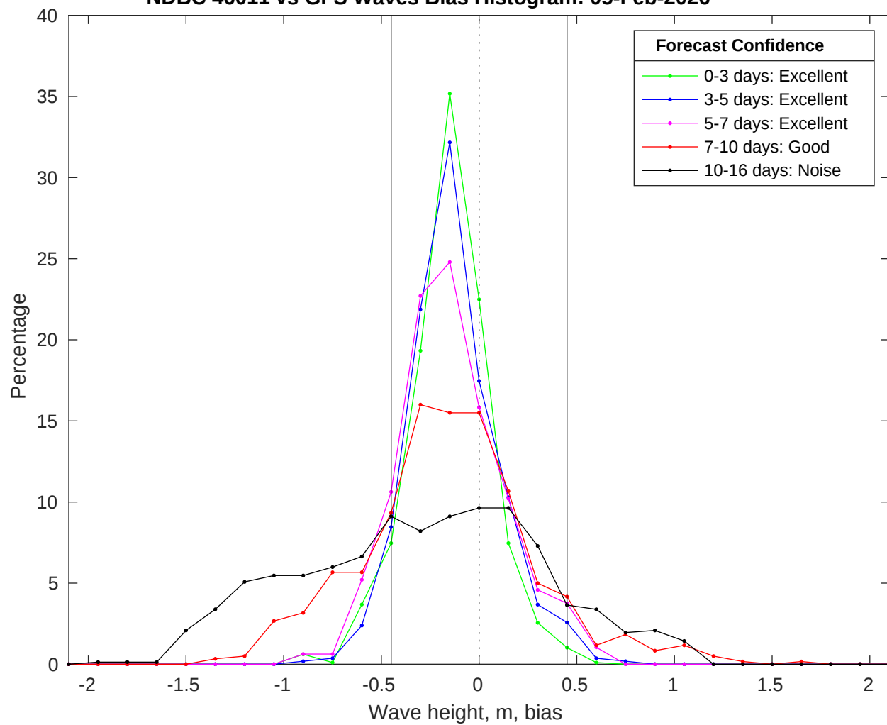
NDBC 46011 vs GFS Waves Bias Histogram: 05-Feb-2026
