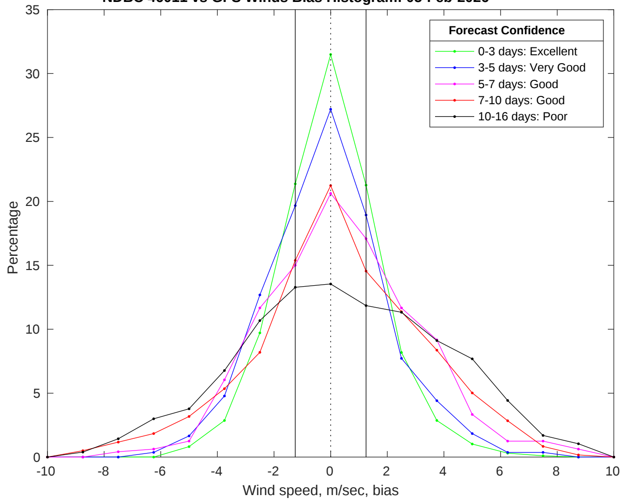
NDBC 46011 vs GFS Winds Bias Histogram: 05-Feb-2026
