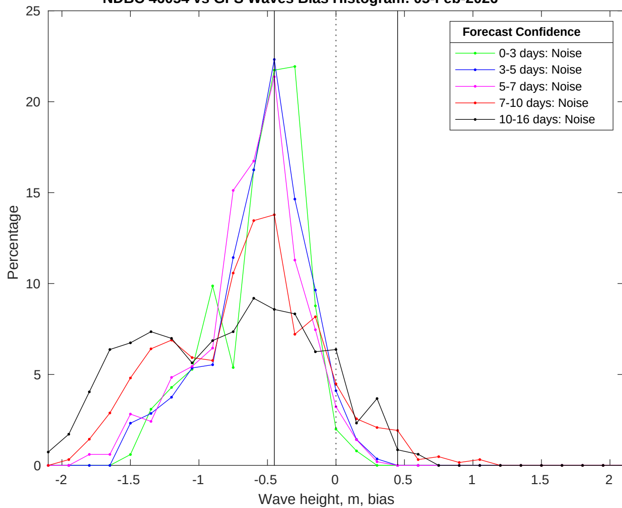
NDBC 46054 vs GFS Waves Bias Histogram: 05-Feb-2026
