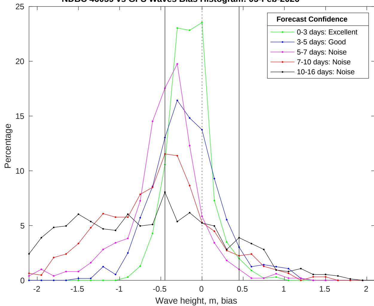
NDBC 46059 vs GFS Waves Bias Histogram: 05-Feb-2026
