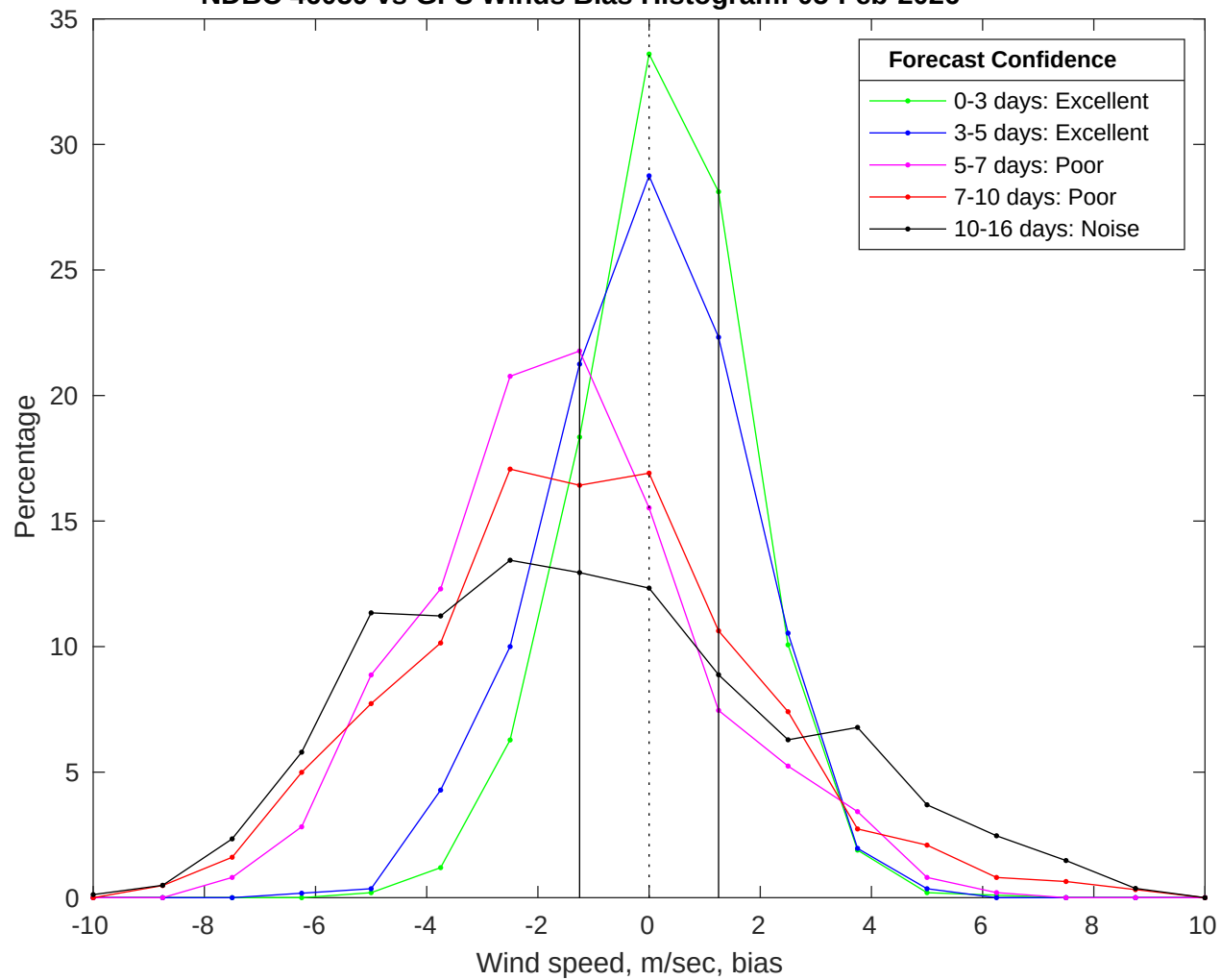
NDBC 46059 vs GFS Winds Bias Histogram: 05-Feb-2026
