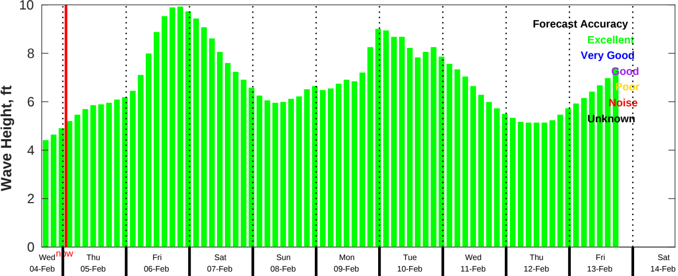
CMEMS Wave Forecast for NDBC 46215 from 04-Feb-2026 16:00:00 to 14-Feb-2026 16:00:00
