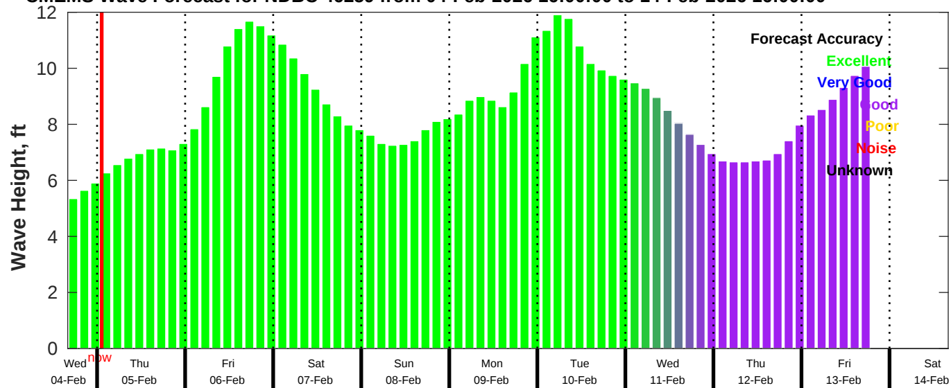
CMEMS Wave Forecast for NDBC 46259 from 04-Feb-2026 16:00:00 to 14-Feb-2026 16:00:00
