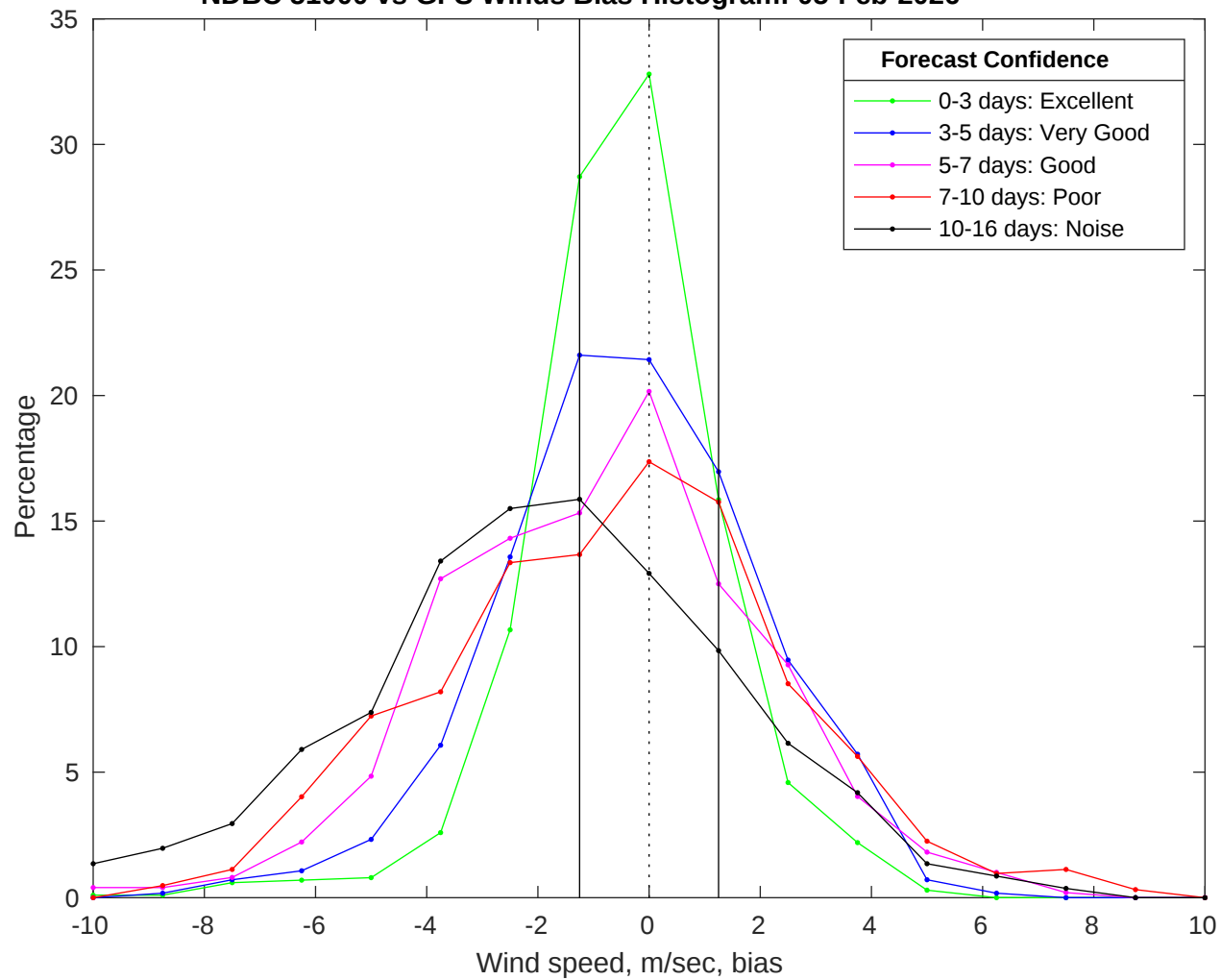
NDBC 51000 vs GFS Winds Bias Histogram: 05-Feb-2026
