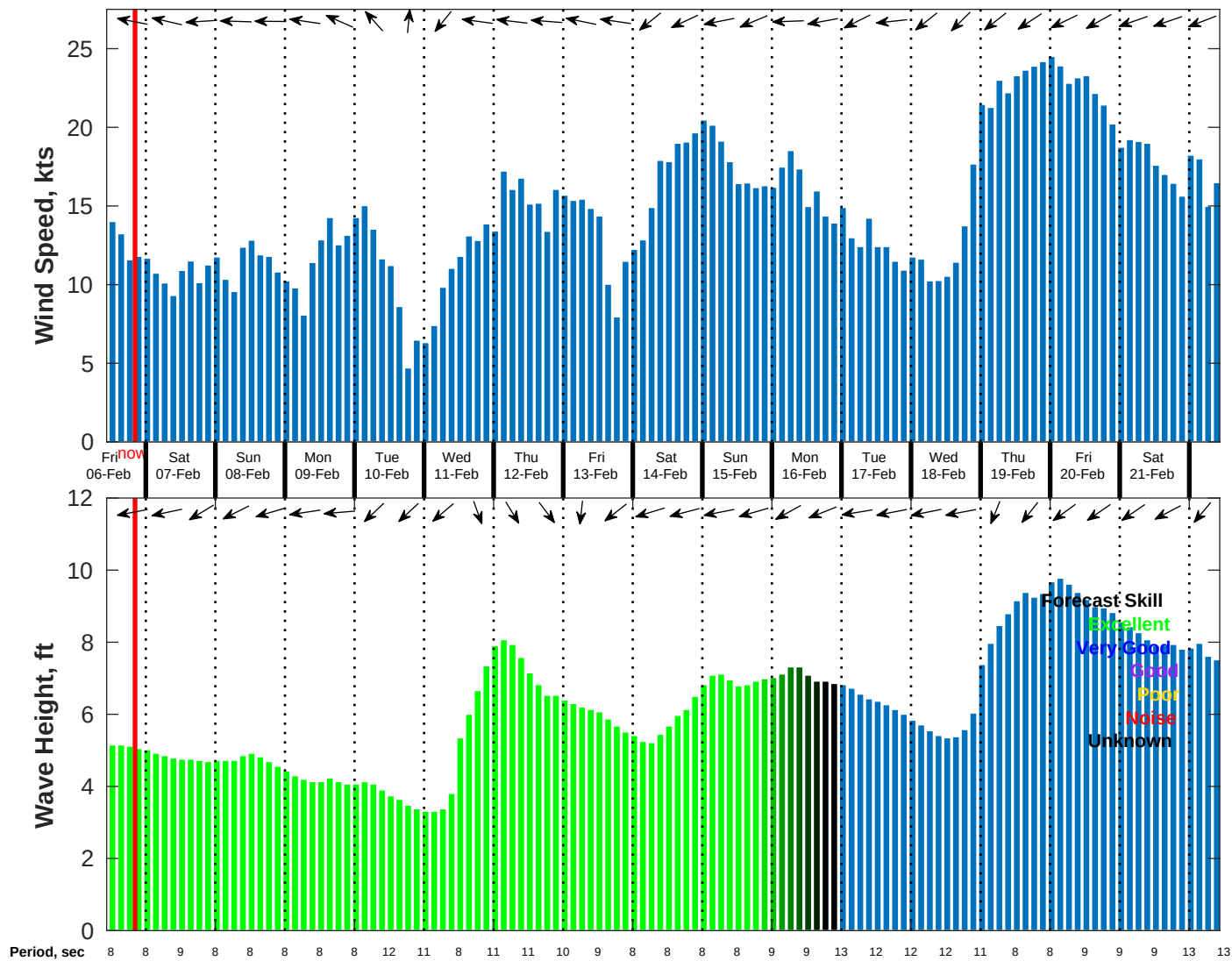
Wind & Wave Forecast for NDBC 52211 from 05-Feb-2026 11:00:00 to 21-Feb-2026 11:00:00
