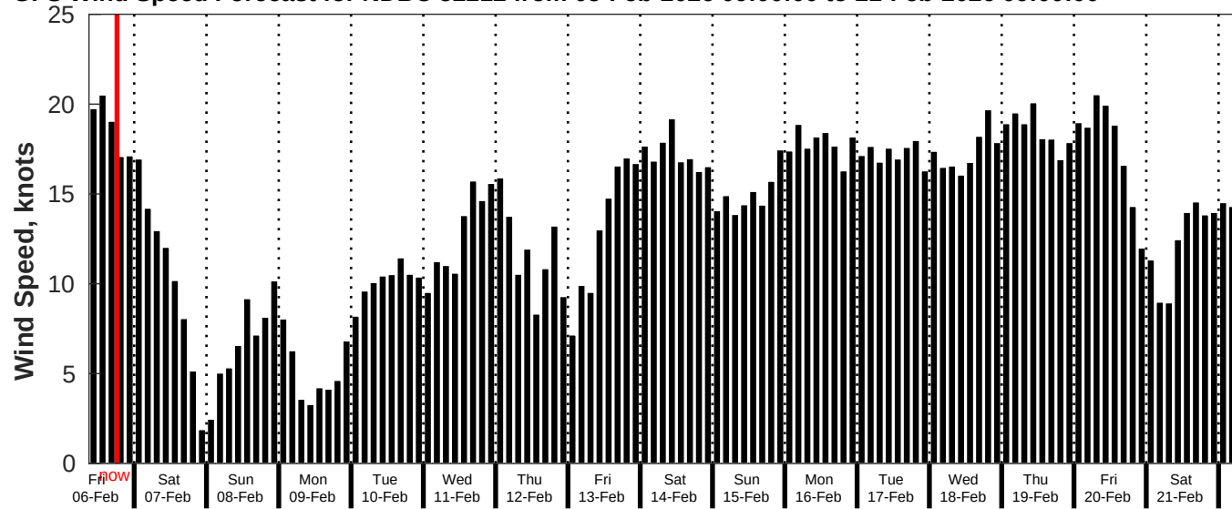
GFS Wind Speed Forecast for NDBC 52212 from 05-Feb-2026 09:00:00 to 21-Feb-2026 09:00:00
