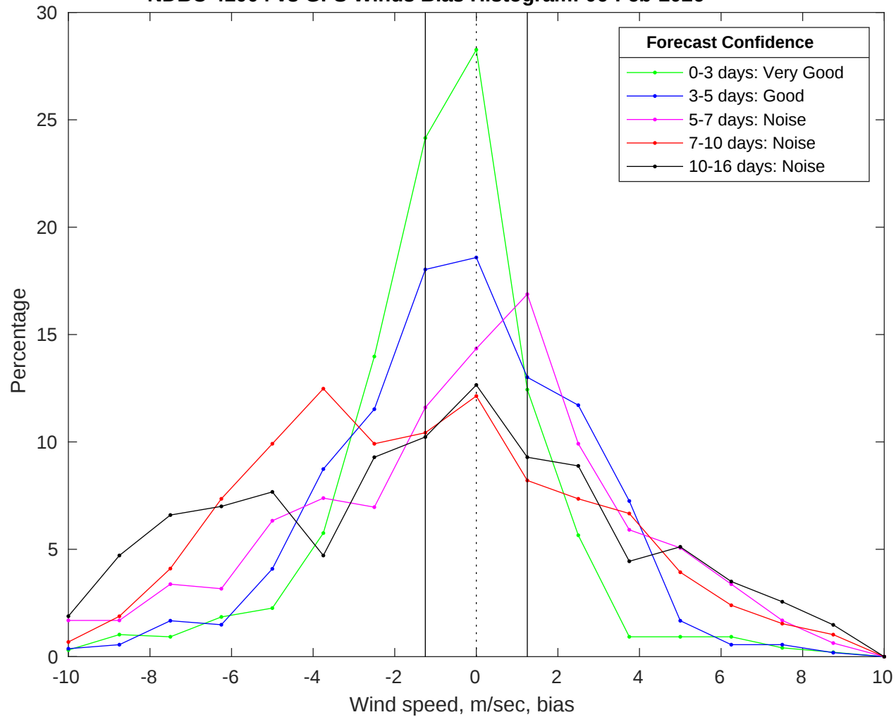
NDBC 41004 vs GFS Winds Bias Histogram: 06-Feb-2026
