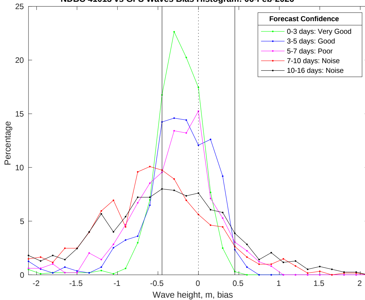
NDBC 41013 vs GFS Waves Bias Histogram: 06-Feb-2026
